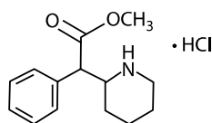
Figure 1: Methylphenidate HCl structure
